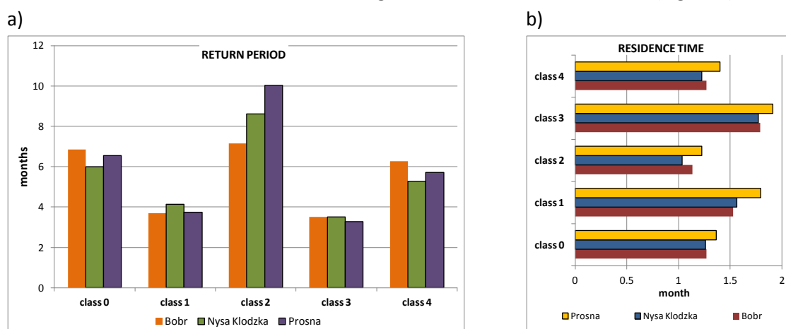
Fig. 13 The return period [months] of each class developed for the locations in Nysa Kłodzka and Prosna river basins Tab.6. The expected residence time of a given SPI-SRI class developed for the locations in Nysa Kłodzka and Prosna river basins
