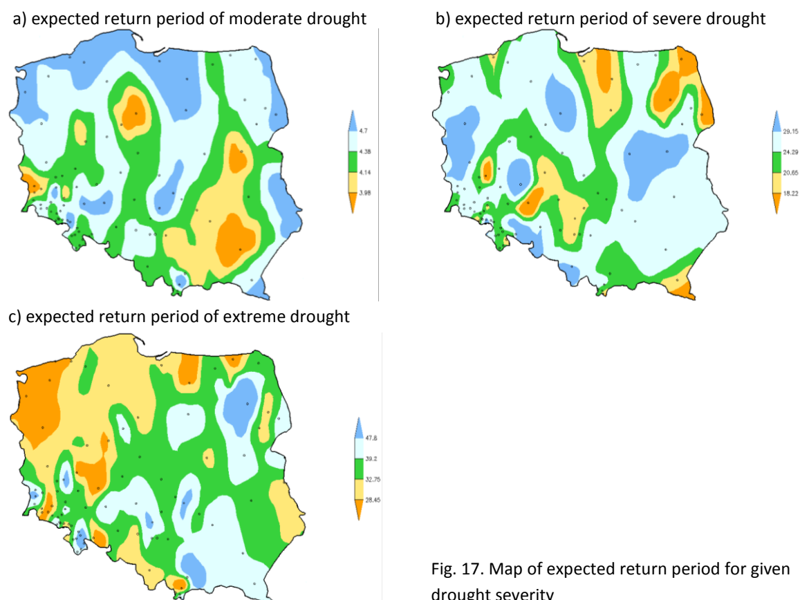
Fig. 16. Map of expected residence time in given drought severity
