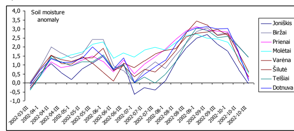
b) SMA in summer season 2002
