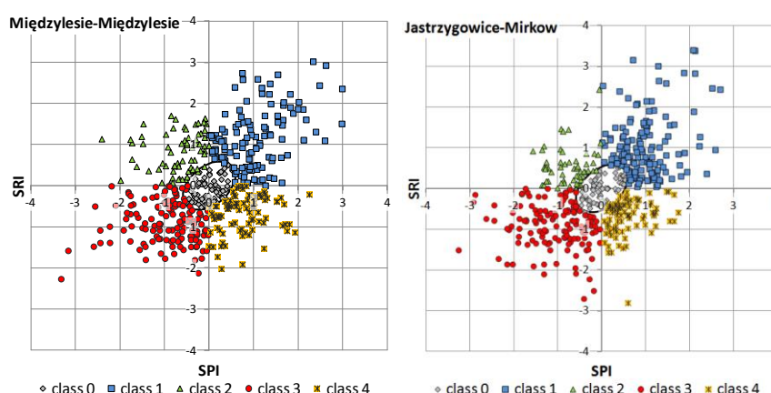
Fig.11. The SPI vs. SRI correlation plots for the coupled meteorological and hydrological stations for a) Nysa Kłodzka and b) Prosna study basin.
