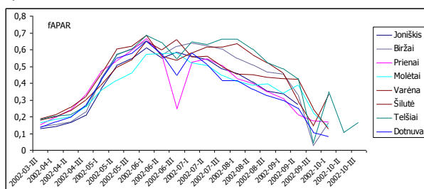
a) fAPAR in summer season 2002
