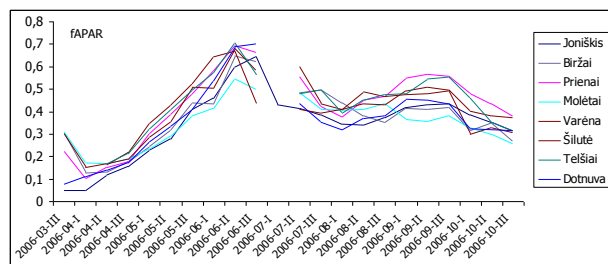
Fig. 3. Fraction of absorbed photosynthetically active radiation (fAPAR) and normalized soil moisture anomaly (SMA) parameters for warm season of 2002 and 2006.
